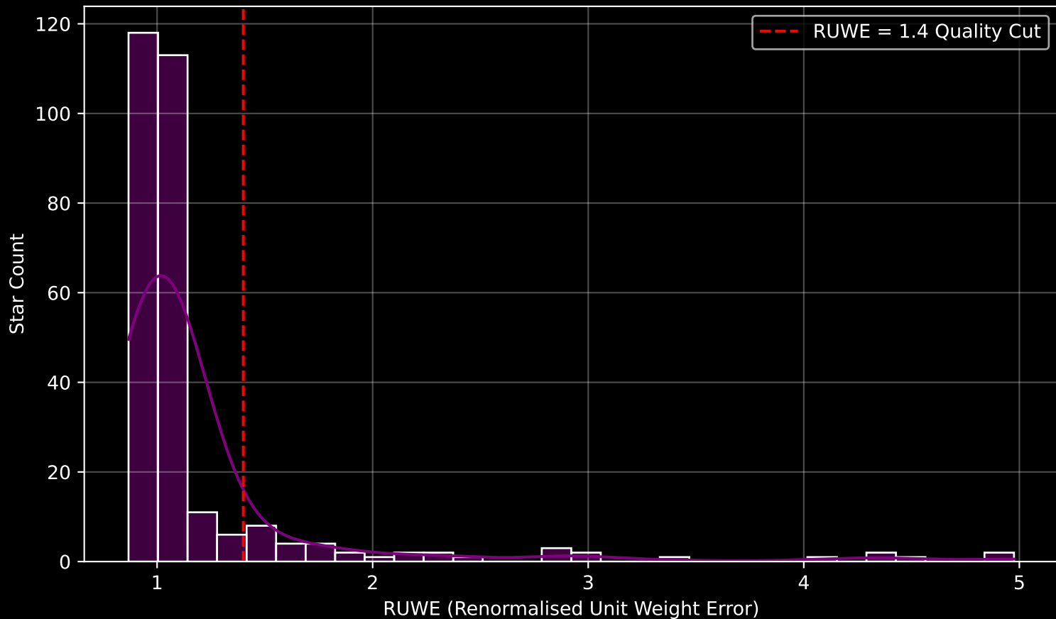
GALAH DR4 Field [6929] RUWE Distribution (n= 284)
