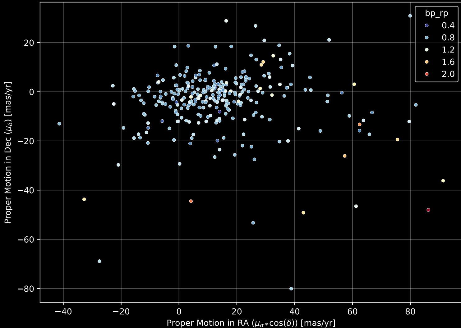
GALAH DR4 Field: [6929] Proper Motion Diagram (n= 292)
