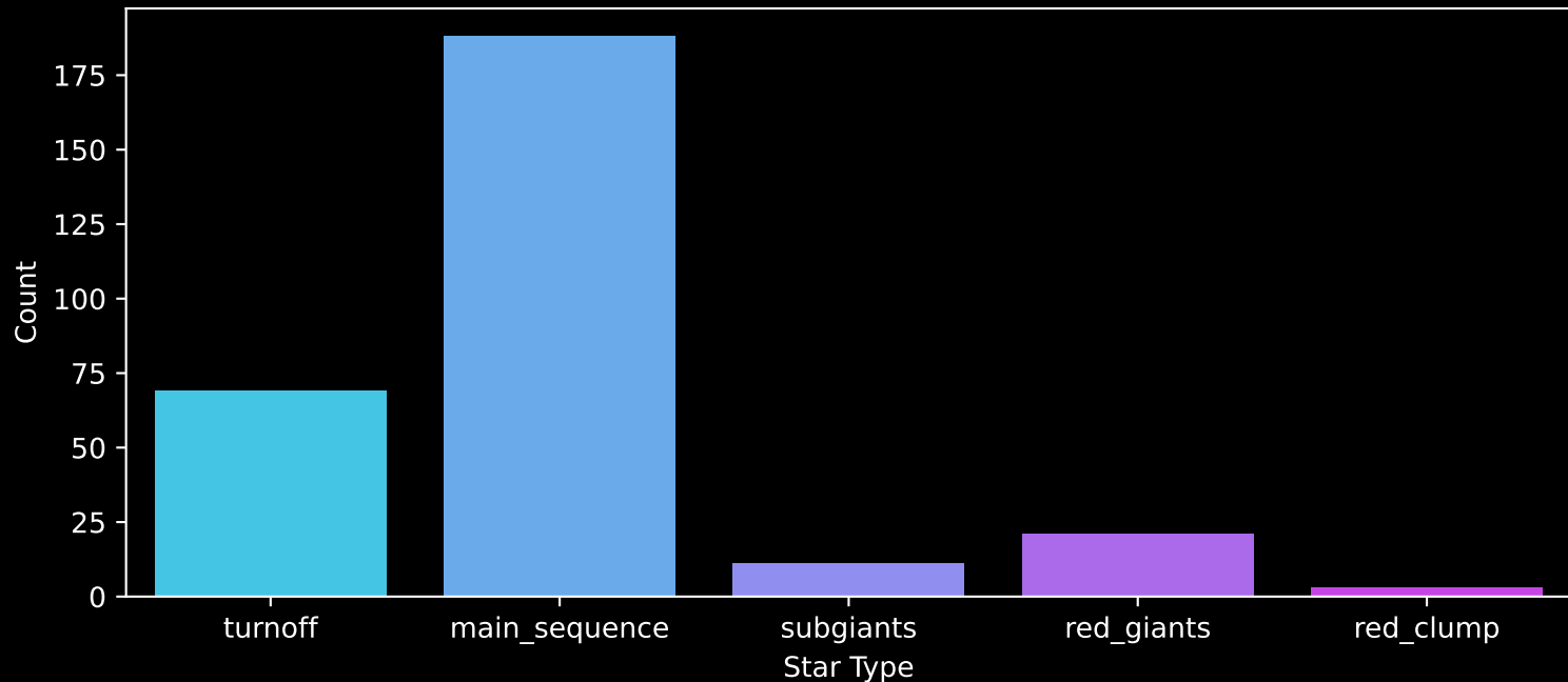
GALAH DR4 Field: [6929] Count plot of Star Type
