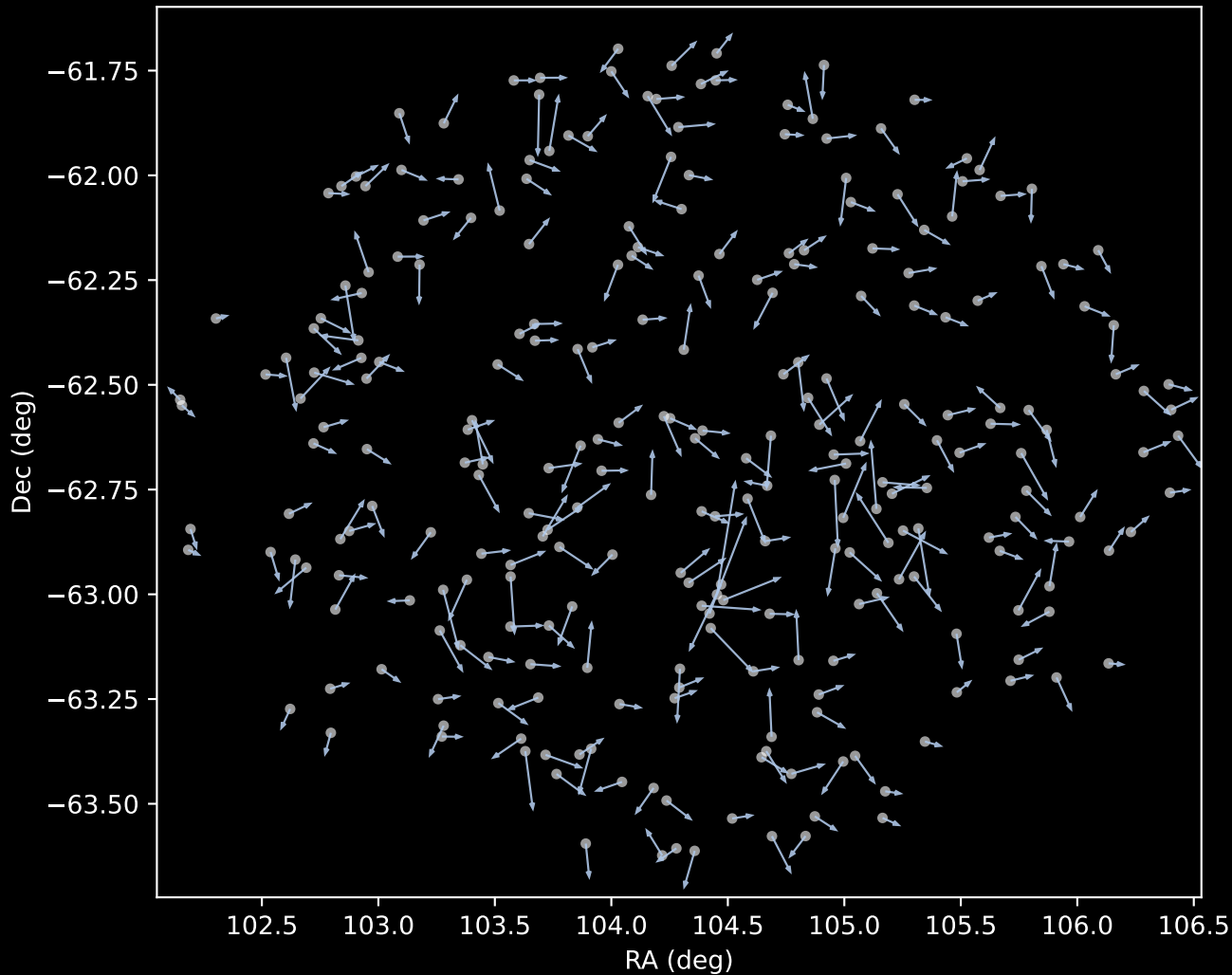
GALAH DR4 Cluster 1 Proper Motion Vectors (n=263)
